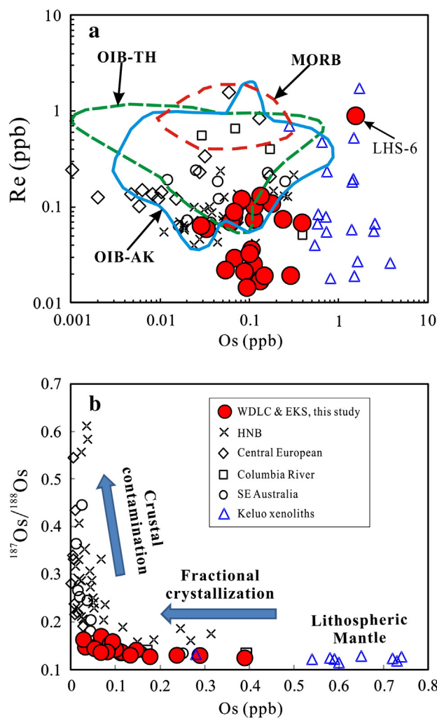
Fig. 5. Re vs. Os (a) and Os concentration vs. ^{187}Os/^{188}Os (b) variation diagrams. Data sources: Central European (Jung et al., 2011); HNB, Hannuoba (Jiang and Zhi, 2010); SE Australia (McBride et al., 2001); Columbia River (Chesley and Ruiz, 1998); Keluo mantle xenoliths (Zhang et al., 2011); MORB and OIB fields are from Shirey and Walker (1998); OIB TH, ocean island basalt tholeiites; OIB AB, ocean island alkali basalts. In (b): Samples with Os > 0.8 ppb are not plotted for clarity; ^{187}Os/^{188}Os ratios are all age-corrected values.
