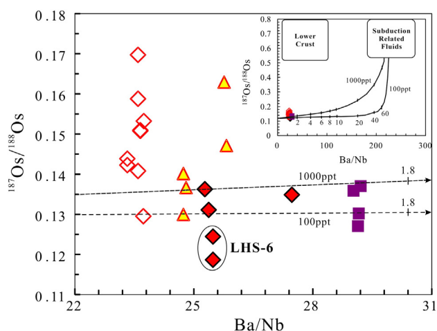
Fig. 10. ^{187}\text{Os}/^{188}\text{Os} vs. \text{Ba}/\text{Nb} for WDLC and EKS basalts. Symbols as in Fig. 8. Trends for contamination of mantle source of basalts by subduction-related fluids, fields of \text{Ba}/\text{Nb} and ^{187}\text{Os}/^{188}\text{Os} for the subduction fluids and the lower crust based on Chesley et al. (2002). Numbers along trend lines represent percentage of fluid required to influence the mantle source. Large numbers along trend lines represent the Os in ppt for subduction-related fluids used in the two-component mixing model (the mantle source of WDLC and EKS basalts is assumed to be 1000 ppt). The real trend should possibly toward more radiogenic Os along with increasing \text{Ba}/\text{Nb} ratios due to the effect of preferential melting of metasomatic components in mantle source for Os isotopes (e.g., Harvey et al., 2011).
