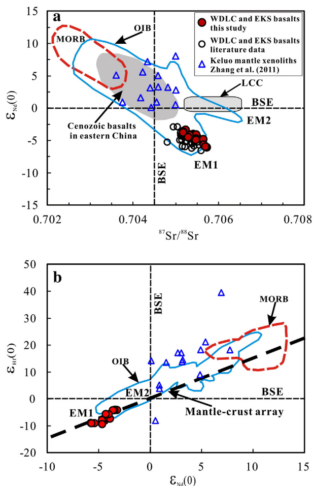
Fig. 4. Sr–Nd (a) and Hf–Nd (b) isotope diagrams for WDLC and EKS basalts. In (a): literature data for WDLC and EKS basalts are from Peng et al. (1986), Basu et al. (1991), Zhang et al. (1995, 1998) and Zou et al. (2003); Field for lower continental crust (LCC) in WDLC and EKS area is based on Wu et al. (2003). Field for Cenozoic basalts in eastern China is based on Chen et al. (2007) and Yan and Zhao (2008); MORB, OIB, BSE, EM1 and EM2 end members are from Zindler and Hart (1986). In (b): MORB and OIB fields are based on Salters and White (1998); the bulk Earth ^{176}Hf/^{177}Hf value (BSE) and the mantle–crust array are based on Blichert-Toft and Albarède (1997).
